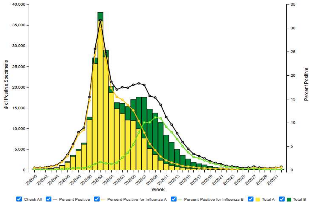
Influenza Positive Tests Reported to CDC by Clinical Laboratories, National Summary, 2025-26 Season, week ending Aug 15, 2026
